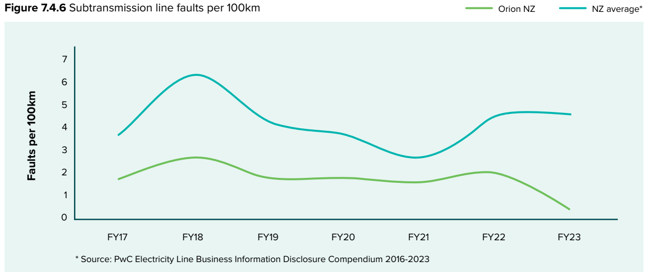
Figure 7.4.6 Subtransmission line faults per 100km
